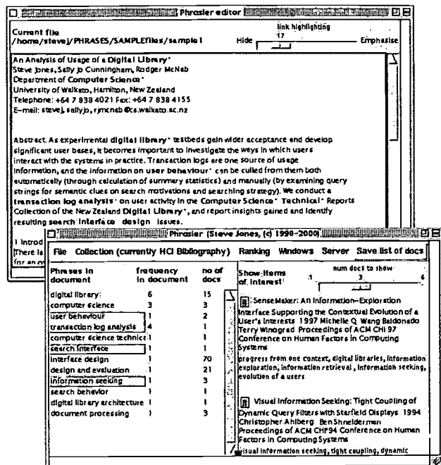
Figure 2: The Phrasier user interface.
